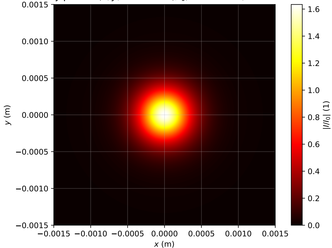
Intensity profile I(x, y, z = 2.229m)/I_0 , Pin=0.9Pcr, artificial time
